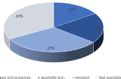
Distribution of sample in the four clusters
